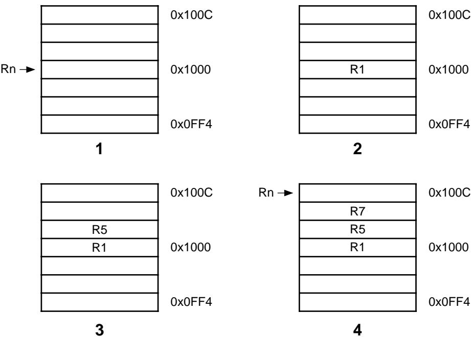
Figure 19: Post-increment addressing
