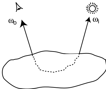
Figure 17.1: The bidirectional scattering-surface reflectance distribution function generalizes the BSDF to account for light that exits the surface at a point other than where it enters. It is more difficult to evaluate than the BSDF, though subsurface light transport can make a substantial contribution to the appearance of many real-world objects.
