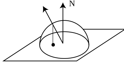
Figure 14.10: Malley's method: to sample direction vectors from a cosine-weighted distribution, uniformly sample points on the unit disk and project them up to the unit sphere.
