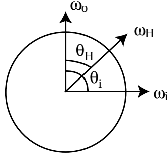
Figure 15.7: The adjustment for change of variable from sampling from the half-angle distribution to sampling from the indicent direction distribution can be derived with an observation about the relative angles involved.
