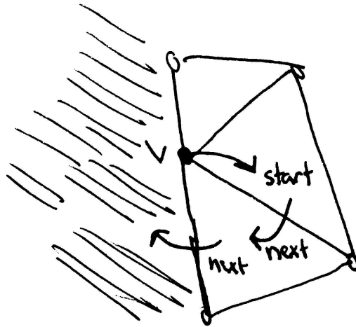
Figure 3.12: We can determine if a vertex is a boundry vertex by starting from the adjacent face startFace and following next face pointers around the vertex. If we come to a face that has no next neighbor face, then the vertex is on a boundary. If we return to startFace , it's an interior vertex.
