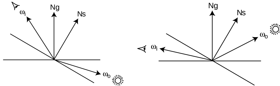
Figure 10.2: The two types of error that result from using shading normals: on the left, a light leak, where the geometric normal indicates that the light is on the back-side of the surface, but the shading normal indicates the light is visible (assuming a reflective and not transmissive surface.) On the right is a dark spot, where the geometric normal indicates that the surface is illuminated but the shading normal indicates that the viewer is behind the lit side of the surface.
