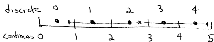
Figure 11.12: The computation to find the first texel inside a reconstruction filter's support is slightly tricky. Consider a filter centered around continuous coordinate 2.75 with width 2, as shown here. The filter's support covers the range [0.75, 4.75] , though texel zero is outside the filter's support: adding 0.5 to the lower end before taking the floor to find the discrete texel gives the correct starting texel, number one.
