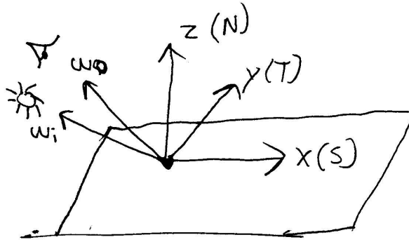
Figure 9.2: basic BSDF interface setting: the shading coordinate system is defined by the orthonormal basis vectors (\mathbf{s}, \mathbf{t}, \mathbf{n}) . We will orient these vectors such that they lie along the x , y , and z axes in this coordinate system. Direction vectors \omega in world space are transformed into the shading coordinate system before any of the BRDF or BTDF methods are called.
