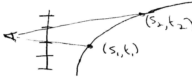
Figure 11.2: Given a set of image samples (here denoted by hash marks on the image plane) at some sampling rate, the 3D scene is sampled at some other rate by the camera rays. If our texture function depends on 2D surface coordinates (s, t) , then the sampling rate in (s, t) can be approximated by the change in sample values ((s_1 - s_2)/2, (t_1 - t_2)/2) between adjacent image sample locations. This texture sampling rate is difficult to compute exactly: it is likely to be varying from sample to sample on the image plane, and it depends on the image sampling rate, the camera imaging model, the geometry of the 3D shape, and the association of (s, t) coordinates with 3D points on the object.
