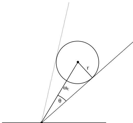
Figure 15.9: To sample points on a spherical light source, we can uniformly sample within the cone of directions around a central vector \omega_c with a angular spread of up to \theta .
