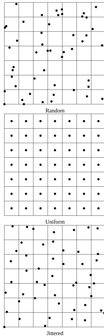
Figure 7.14: Three 2D sampling patterns. The random pattern on the top is a poor pattern, with many clumps of samples that leave large sections of the image poorly sampled. In the middle is a uniform stratified pattern which is better distributed but can exacerbate aliasing artifacts. On the bottom is a stratified jittered pattern, which turns aliasing from the uniform pattern into high-frequency noise while still maintaining the benefits of stratification.
