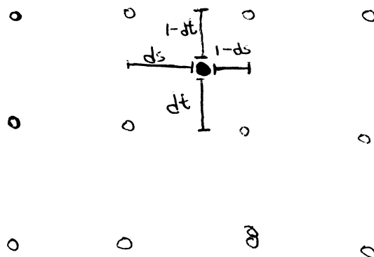
Figure 11.14: To compute the value of the image texture function at an arbitrary (s, t) position, MIPMap::triangle() finds the four texels around (s, t) and weights them according to a triangle filter based on their distance to (s, t) . One way to implement this is as a series of linear interpolations, as shown here: first, the two texels below (s, t) are linearly interpolated to find a value at (s, 0) , and the two texels above it are interpolated to find (s, 1) . Then, (s, 0) and (s, 1) are linearly interpolated again to find the value at (s, t) .
