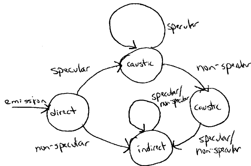
Figure 16.11: photon fsm
