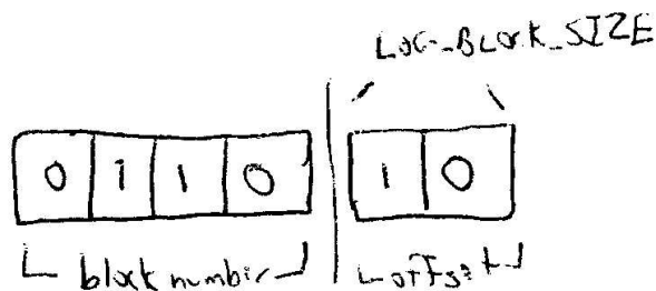
Figure A.3: Given an array coordinate, the (u, v) block number that it is in can be found by shifting off the \logBlockSize low order bits for both u and v . (For example, with a \logBlockSize of 2 and thus a block size of 4, we can see that this correctly maps 1D array positions from 0 to 3 to block 0, 4 to 7 to block 1, etc. To find the offset within the particular block, we just mask off the high order bits, leaving the \logBlockSize low order bits. Because the block size is a power of two, these computations can all be done with a few efficient bit operations.
