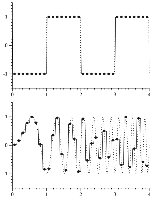
Figure 7.28: The box filter in action, reconstructing samples of the step function (top) and a sinusoidal function with increasing frequency as x increases. It does reasonably well with the step function (as would be expected), but an extremely poor job with the sinusoidal function.
