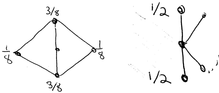
Figure 3.17: Subdivision rule for edge split: the position of the new odd vertex, marked with an “x” (what?) , is found by weighting the two vertices at the ends of the edge and the two vertices opposite it on the adjacent triangles. On the left are the weights for an interior vertex; on the right are the weights for a boundary vertex.
