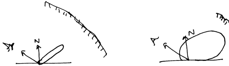
Figure 16.1: sample BSDF vs. sample light..
