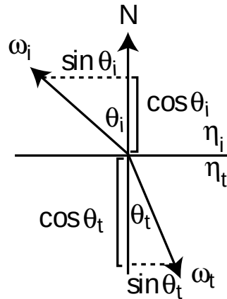
Figure 9.9: Basic geometry for computing the transmitted direction \omega_t from the incident direction \omega_i . The \cos \theta terms are equal to the z components of the direction vectors and the \sin \theta terms are equal to the xy lengths of the corresponding direction vectors.
