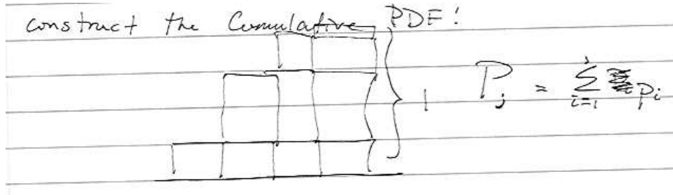
Figure 14.2: A discrete CDF.
