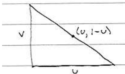
Figure 14.11: Sampling an isosceles right triangle. Note that the equation of the hypotenuse is v = 1 - u .
