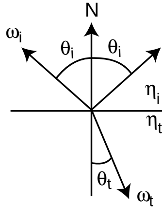
Figure 9.4: Basic setting for specular reflection and transmission. Why isn't w_r labeled in this diagram? The reflected direction \omega_r is the direction \omega_i opposite the outgoing direction \omega_o that makes the same angle \theta_i with the surface normal as the incident ray. The transmitted direction makes an angle \theta_t with the negated surface normal, where \theta_t is given by Snell's law, which depends on the indices of refraction of the incident and transmitted media, \eta_o and \eta_t , respectively.
