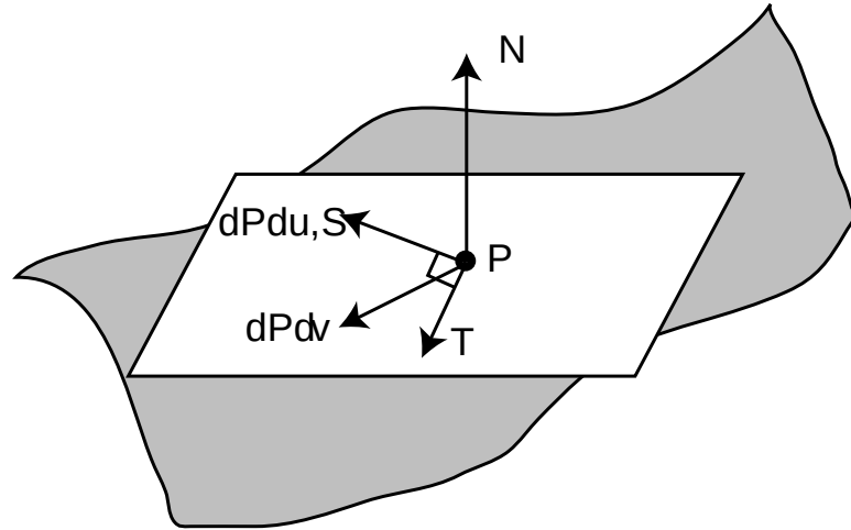
Figure 2.13: The local differential geometry around a point p . The tangent vectors \mathbf{s} and \mathbf{t} are orthogonal vectors in the plane that is tangent to the surface at p . The parametric partial derivatives of the surface, \partial p / \partial u and \partial p / \partial v , also lie in the tangent plane but are not necessarily orthogonal. The surface normal \mathbf{n} , is given by the cross product of \partial p / \partial u and \partial p / \partial v . The vectors \partial \mathbf{n} / \partial u and \partial \mathbf{n} / \partial v (not shown here) record the differential change in surface normal as we move in u and v along the surface.
