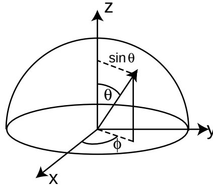
Figure 9.3: As was done for the SpecularTransmission BTDF, the \sin \theta term is found by computing the length of the dashed line, which is the magnitude of the xy components of the vector. The \sin \phi and \cos \phi terms can be computed using the circular coordinate equations x = r \cos \phi and y = r \sin \phi , where r , the length of the dashed line, was already computed for \sin \theta .
