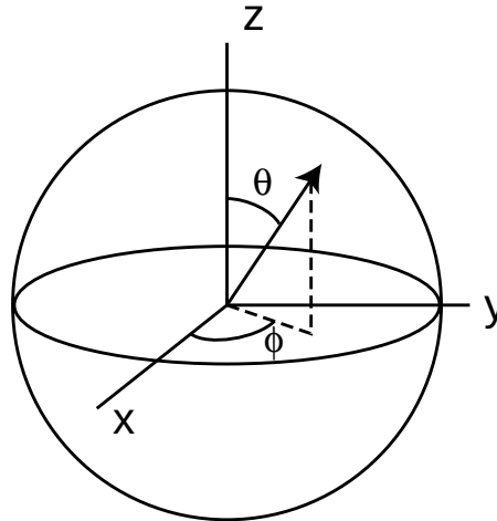
Figure 5.9: A given direction vector can be written in terms of spherical coordinates (\theta, \phi) if the x, y , and z basis vectors are given as well. The spherical angle formulae make it easy to convert between the two representations.
