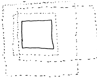
Figure 4.11: No useful splits possible due to overlap. Three bounding boxes overlap the node, yet none of their edges are inside it.
