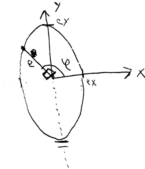
Figure 9.15: The two exponents e_x and e_y for the anisotropic microfacet distribution function give specular exponents for microfacets facing exactly along the x and y axes, respectively. For microfacets with other orientations, the exponent e is computed by finding the radius e of the super-ellipse for the actual orientation angle \phi .
