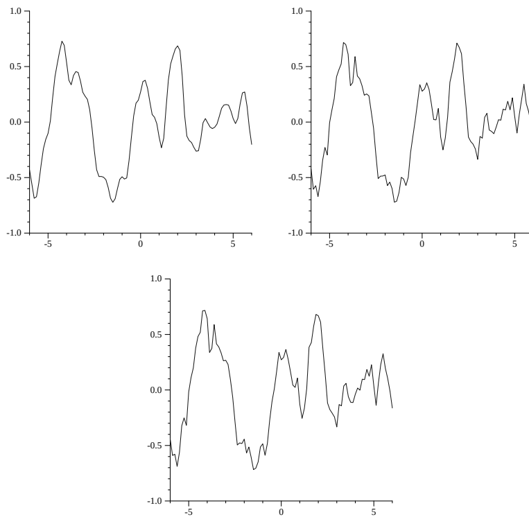
Figure 11.24: Graphs of the \text{FBM}() function for 2, 4, and 6 octaves of noise. Notice how as more levels of noise are added, the graph has progressively more detail, though its overall shape remains roughly the same.
