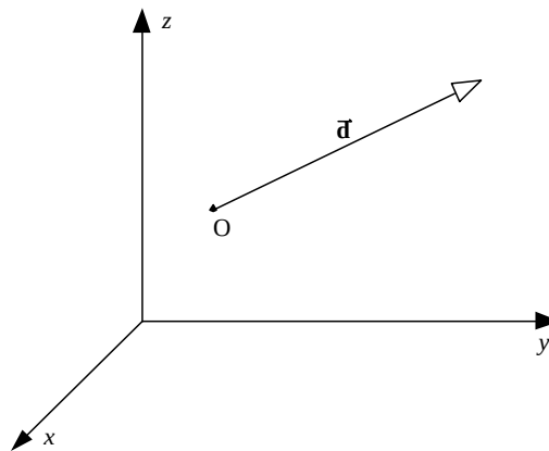
Figure 2.6: A ray is a semi-infinite line defined by its origin o(r) and its direction d(r) .
