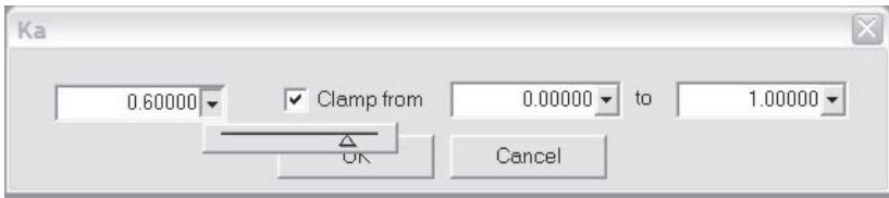
Figure 25: Scalar editor
