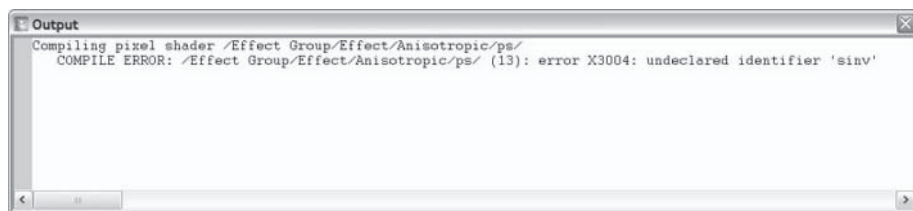
Figure 18: Output window
