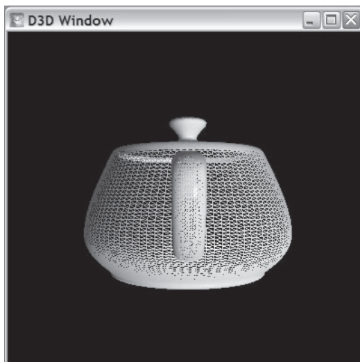
Figure 32: Wireframe display
