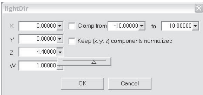
Figure 26: Vector editor
