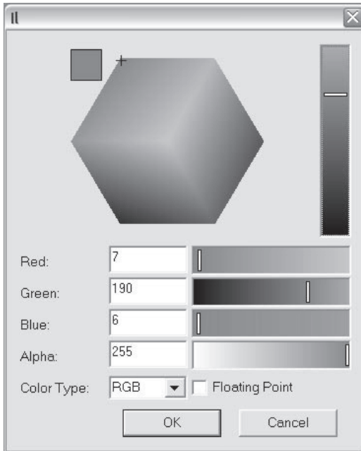
Figure 28: Color editor
